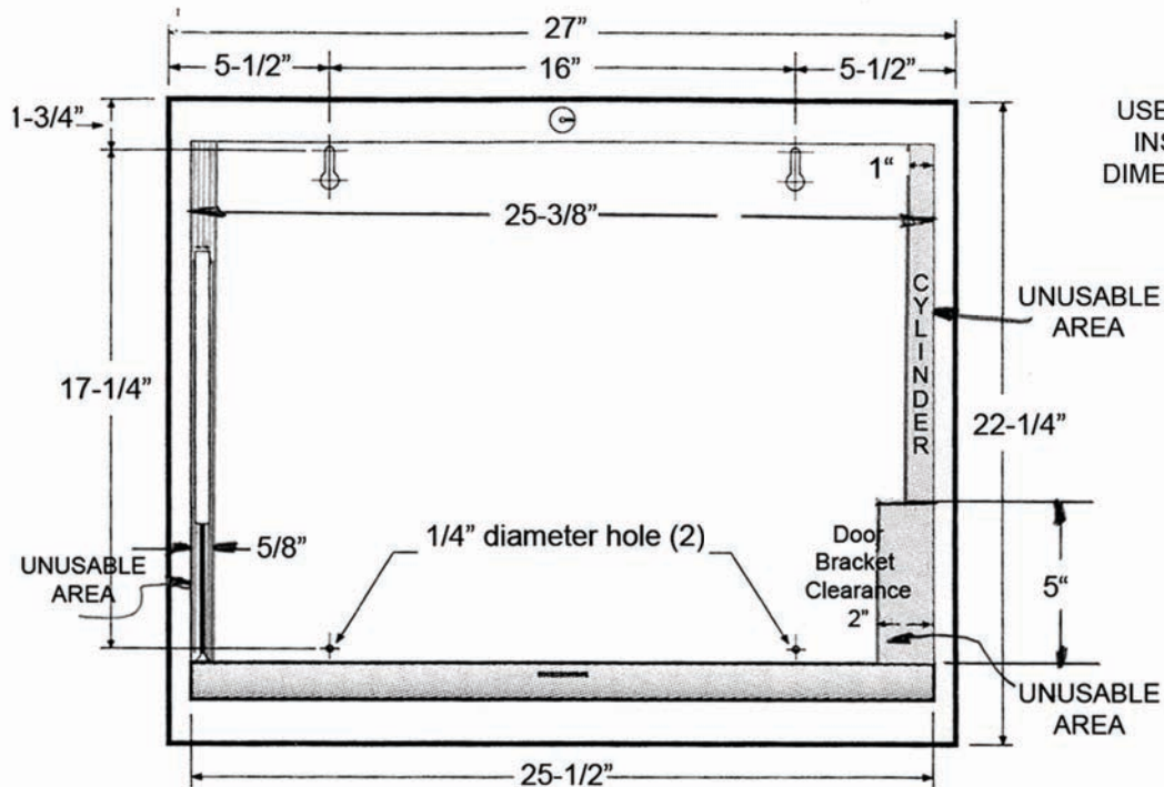
ORIGINAL WALLAROO Front View/Open
