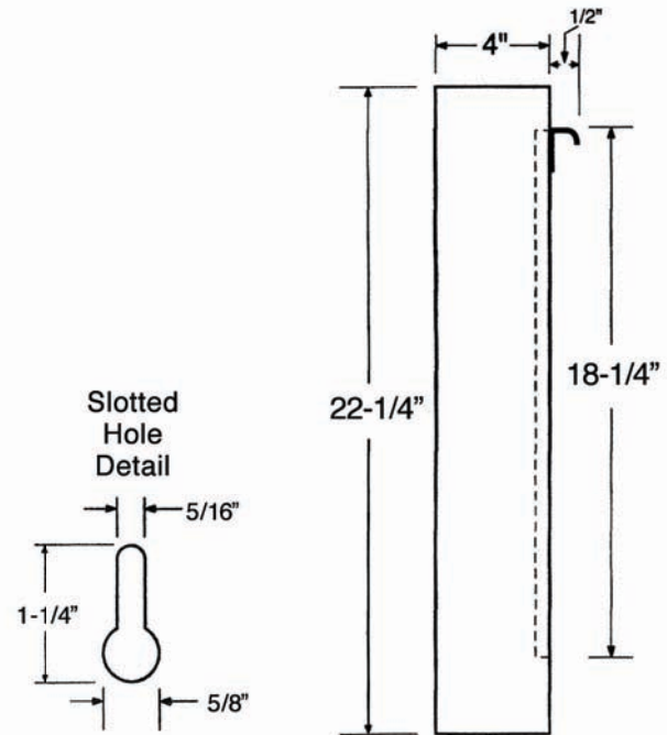
ORIGINAL WALLAROO Side View/Closed (Extruded Handle)
