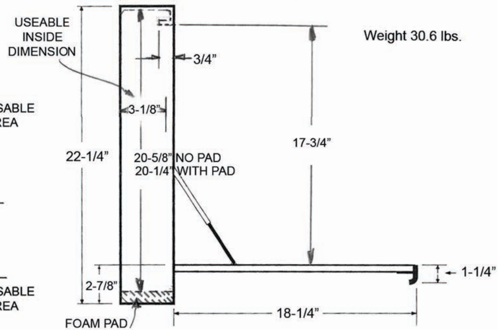
ORIGINAL WALLAROO Side View/Open
