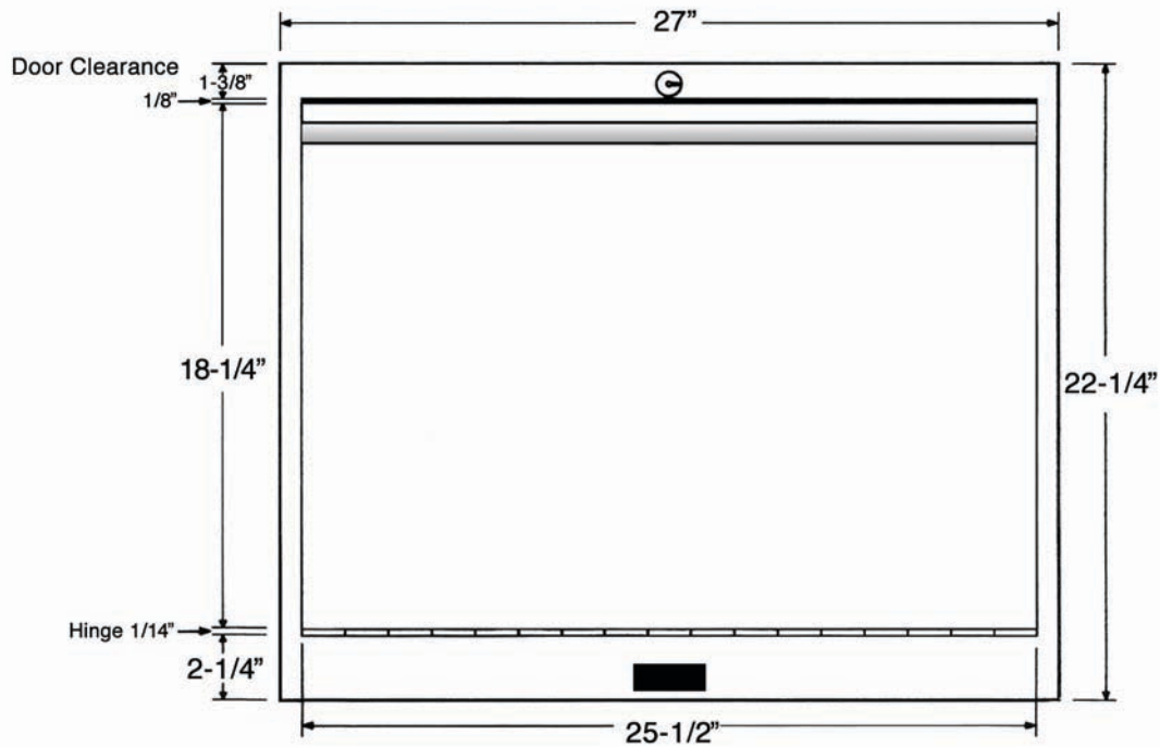
ORIGINAL WALLAROO Front View/Open
