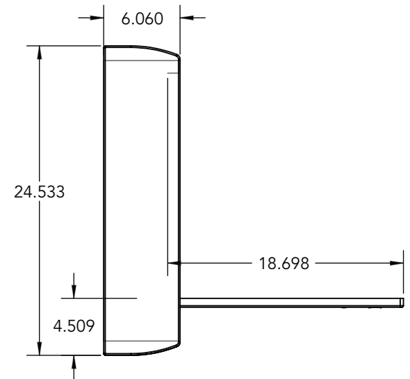
WALLaroo 2000 XD Side View/Open Recessed Handle)
