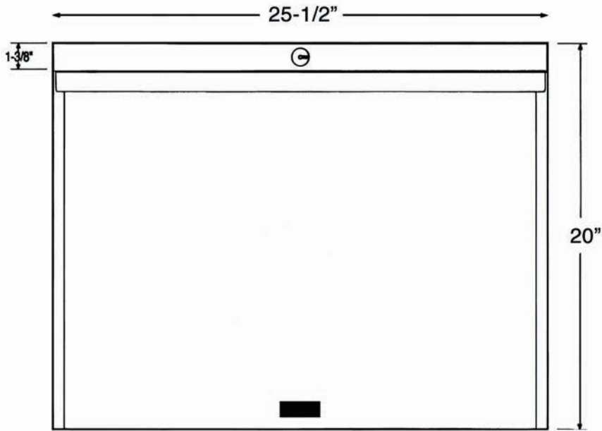
ECONOROO Front View/Open
