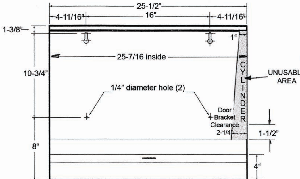
ECONOROO Front View/Open
