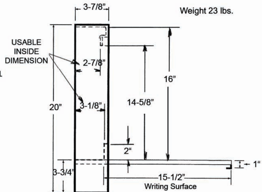
ECONOROO Side View/Open
