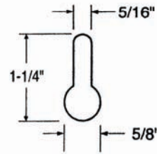
Slotted Hole Detail
